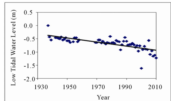
Figure 6. Trend in annual minimum low tidal water levels.
