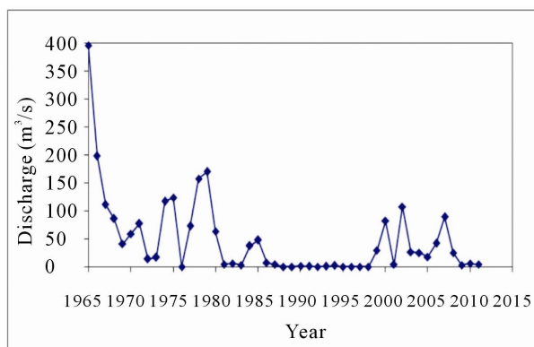
Figure 7. Time series plot of annual lowest flow of the Gorai River at Gorai Railway Bridge.
