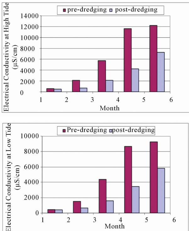
Figure 8. Comparison of Electrical Conductivity (EC) of the Rupsa-Pasur River at Khulna between the pre- and post-dredging situations.
